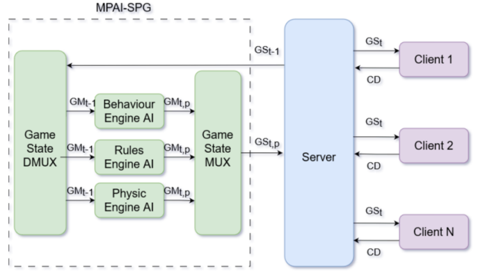
Fig. 1. MPAI-SPG architecture
